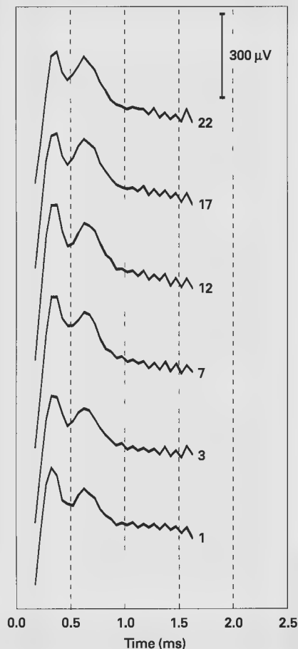
Fig. 8. Recording series with monopolar (MP1) stimuli were presented at electrode 10 (25 \mu s phase width, 224 current level units) and recorded at 6 different sites (electrodes 1, 3, 7, 12, 17, 22) along the array in the monopolar (MP2) configuration. The NRT waveforms show slight differences in response amplitude but no changes in the response waveform category as a function of recording site.
