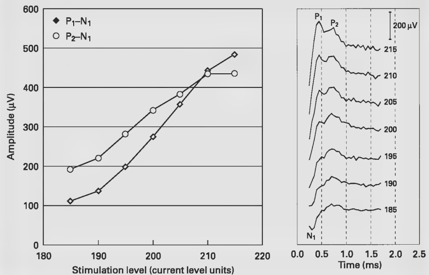
Fig. 7. NRT amplitude growth functions of the P 1 and P 2 peaks. Note also how the response waveform changes from category Ia to category II with increasing stimulation level.
